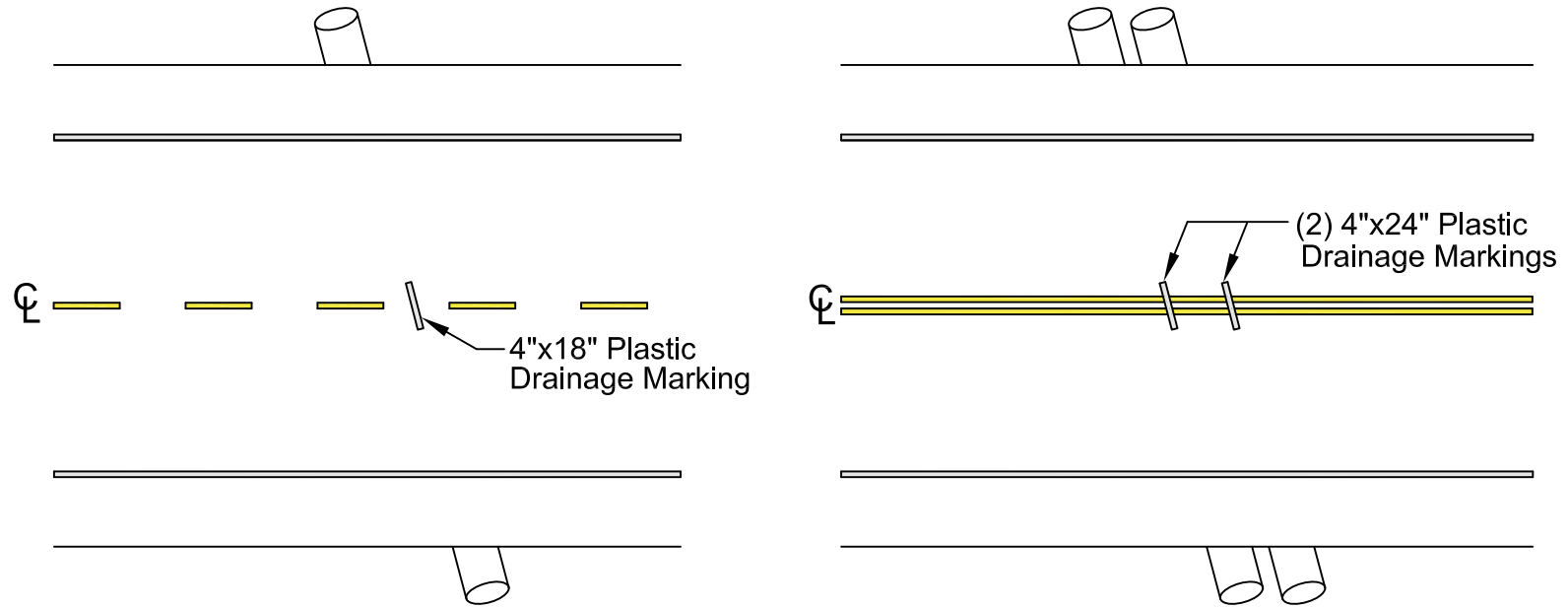
CULVERT DRAINAGE MARKING DETAIL
